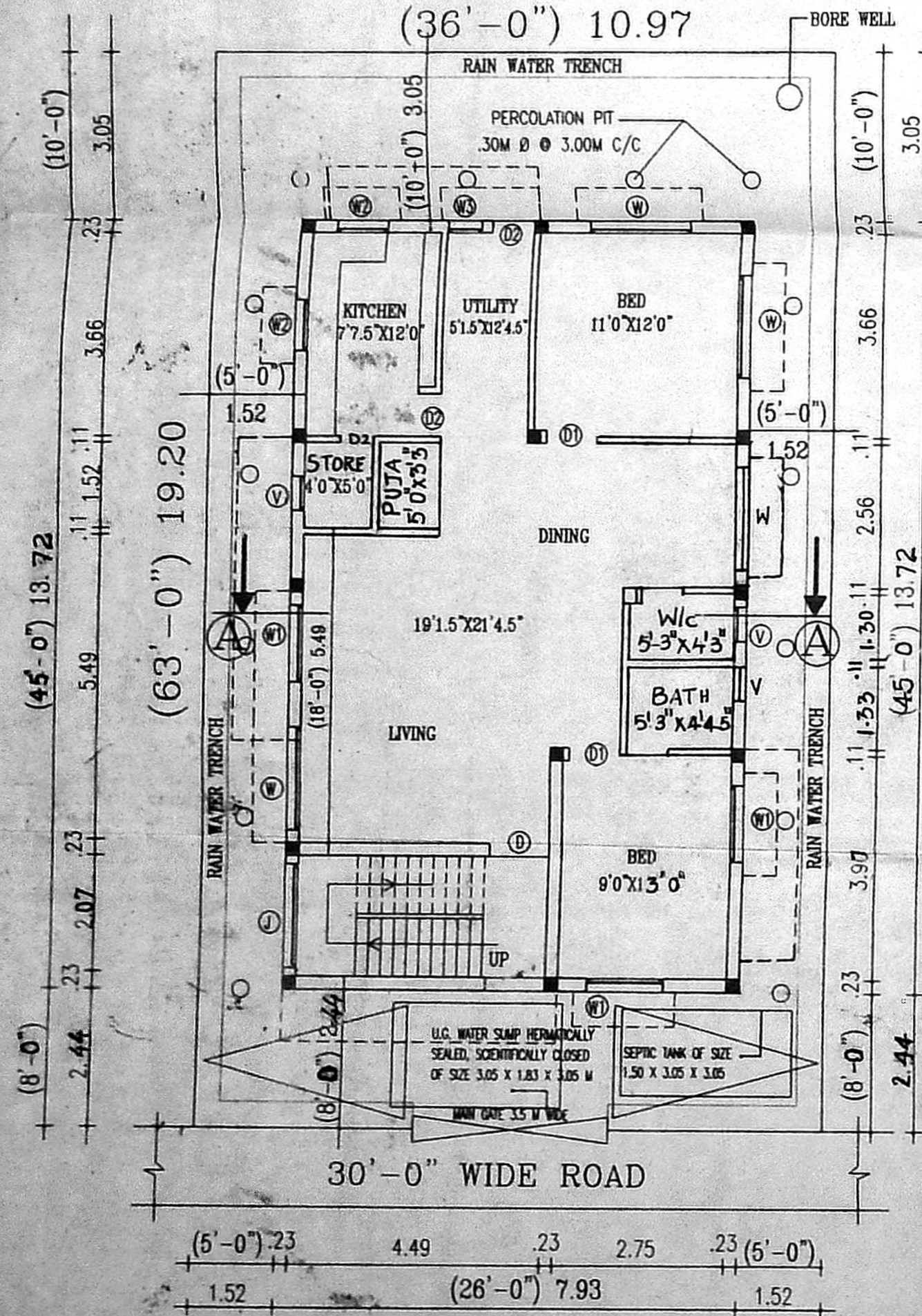
GROUND FLOOR/SITE PLAN
